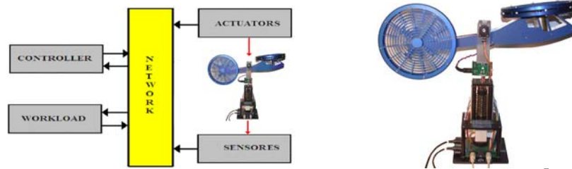
Figure 7. Networked Control System with workload.
