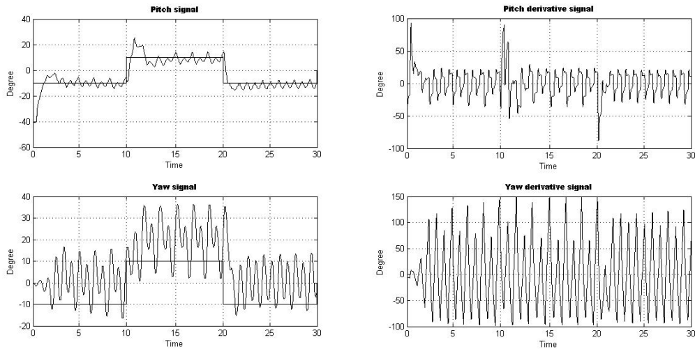
Figure 8. Response of 2-DOF Helicopter. Pitch and Yaw angles and derivatives.
