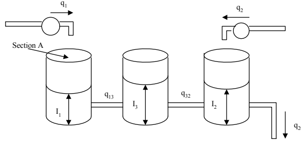
Figure 3. Three tanks representation.
