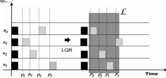
Figure 2. Task periods controlled by LQR controller into a schedulable region.
