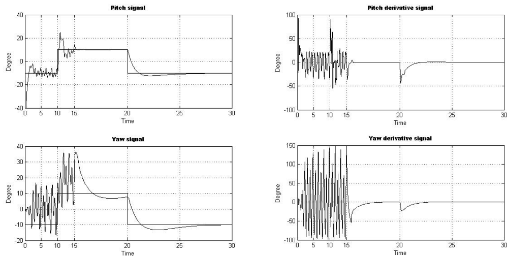
Figure 9. Response of 2-DOF Helicopter. Pitch and Yaw angles and derivatives using frequency transition model.
